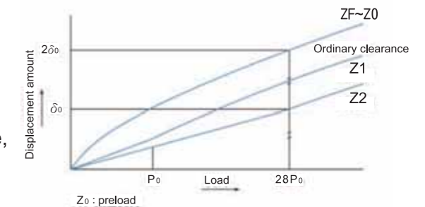
Fig1.10.2 Rigidity Data
